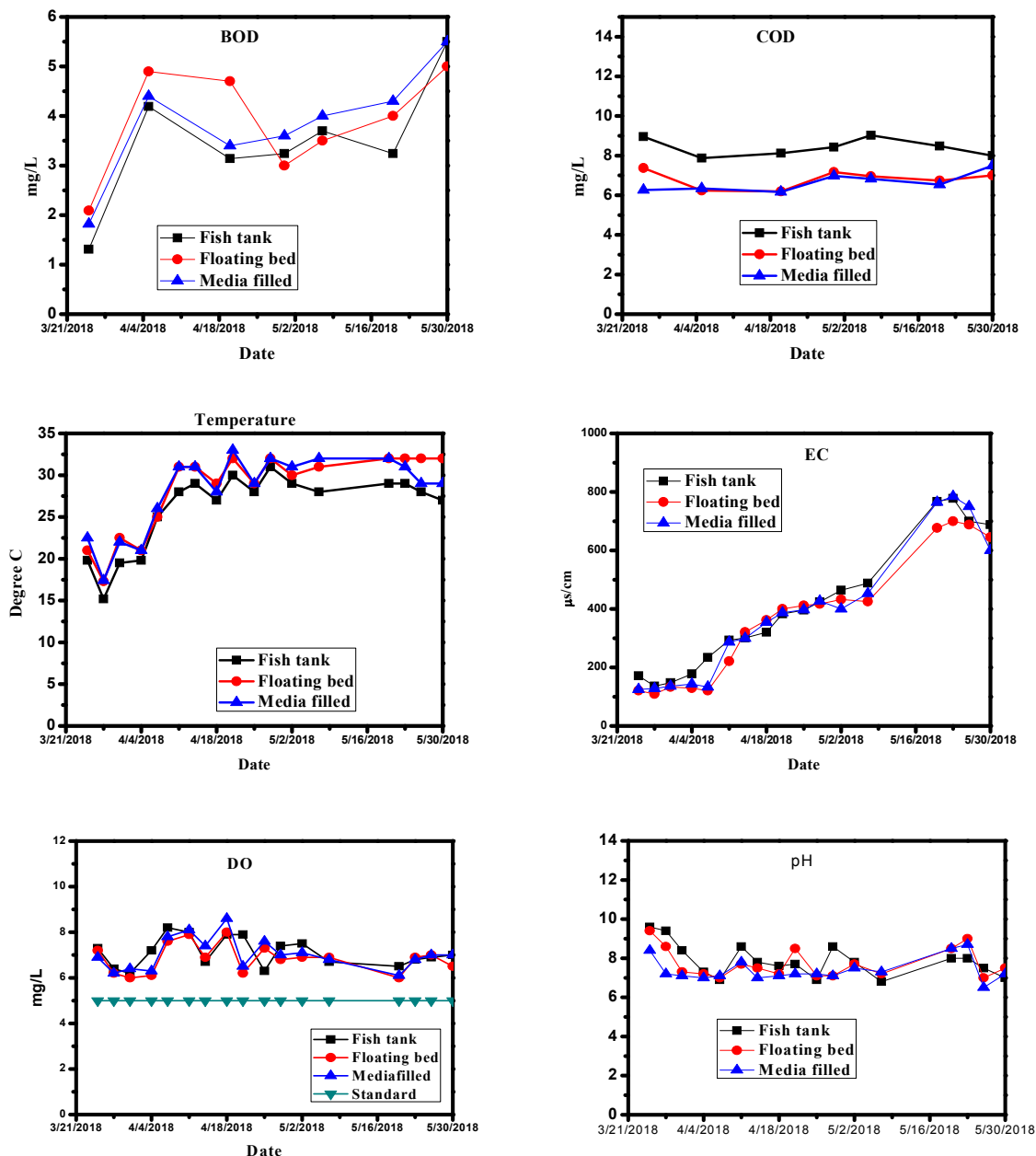
Figure 5. Concentration of COD, BOD, EC, DO, pH, Temperature in The Media Filled System (MFS), Floating Bed Systems (FBS) and Fish Tanks
